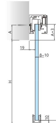
SDS-C01_A wall mounted
