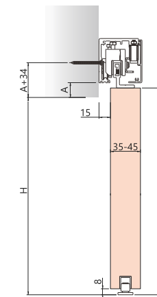
SDS-C01_B wall mounted
