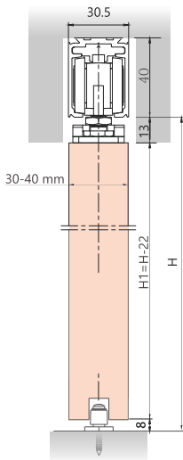
SDS-U01C_A3 with easy clamp
