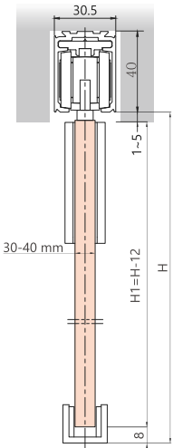
SDS-U01C_A1 with smart clamp
