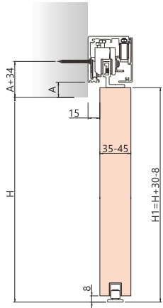
SDS-C01_D wall mounted
