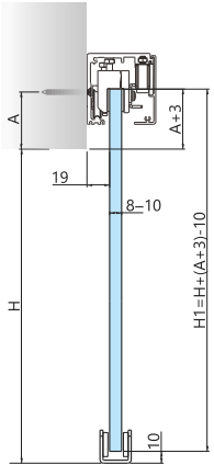
SDS-C01_C wall mounted
