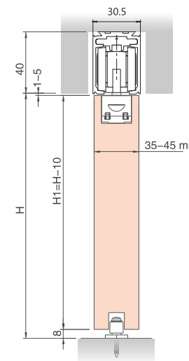
SDS-U01B_A2 with smart box
